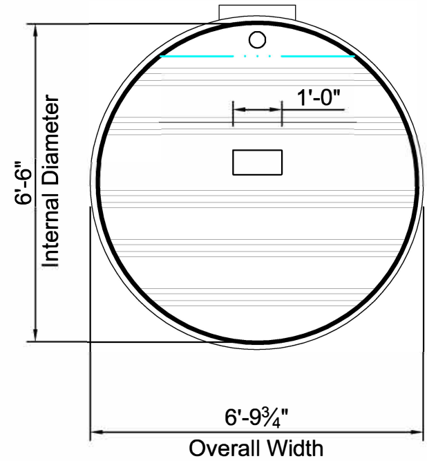
Cross Section
